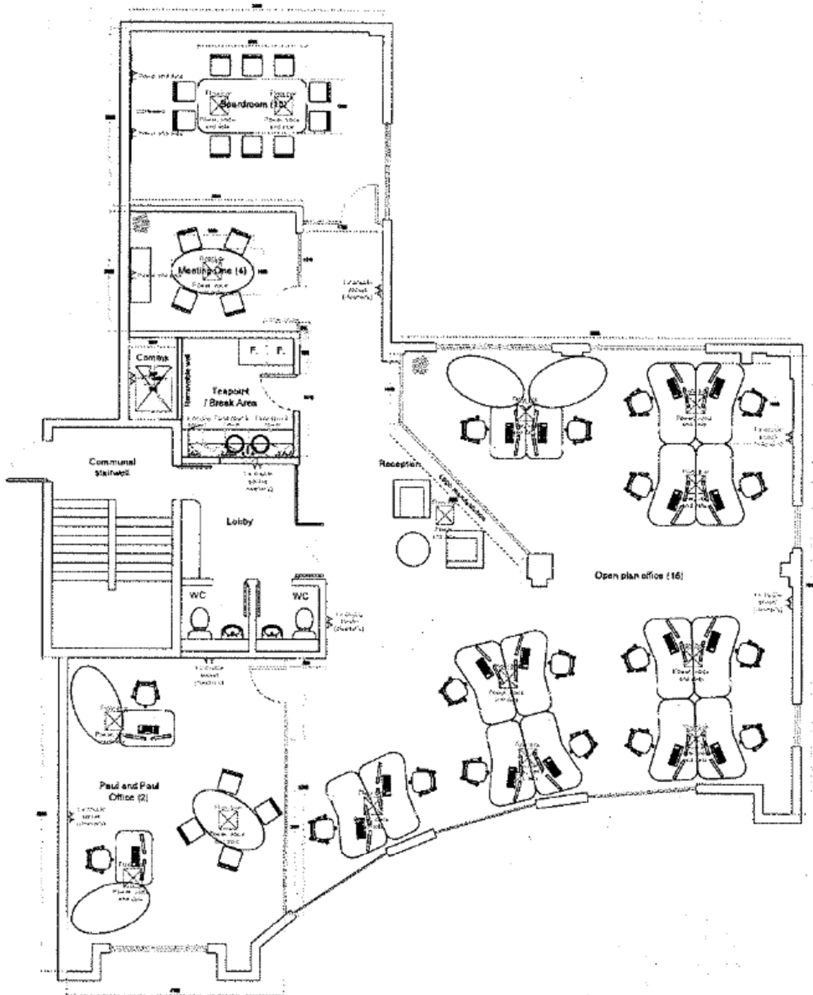
Calico House - Proposed layout
